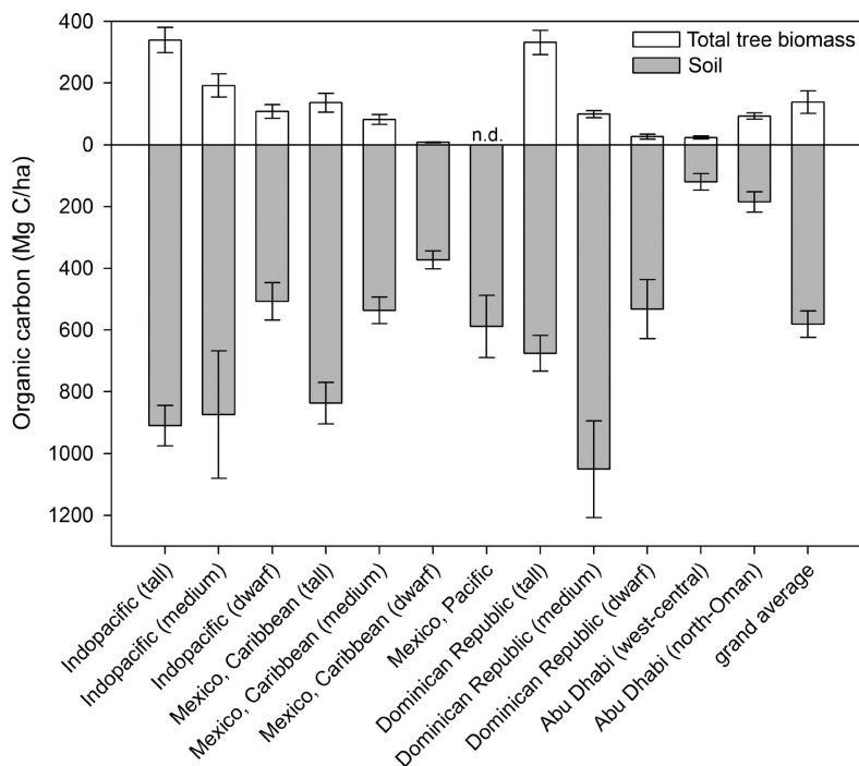
FIG. 4. Global carbon stock comparison for mangroves (source data: Indopacific [Donato et al. 2011, Muriyarso et al. 2015], Mexico, Caribbean [Adame et al. 2013], Mexico, Pacific [Ezcurra et al. 2016], Dominican Republic [Kauffman et al. 2014]; Appendix S2: Table S3) Values are mean \pm SE, n.d. = no data.
