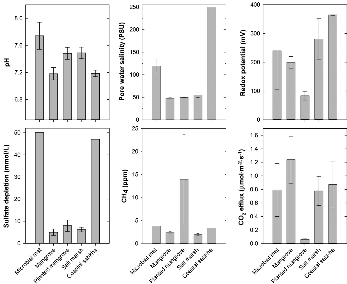
FIG. 7. Pore water chemistry, CO 2 flux, and redox potential data for intertidal ecosystems. Values are mean \pm SE.
